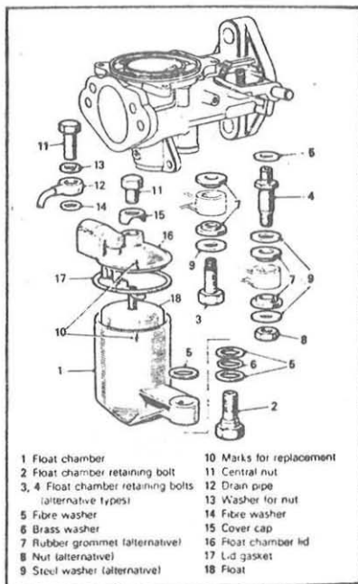
The float chamber components of an H2 carburettor
