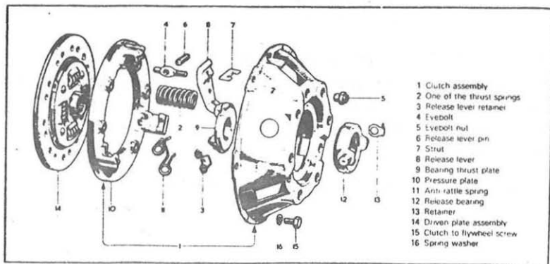
The coil spring clutch completely dismantled
